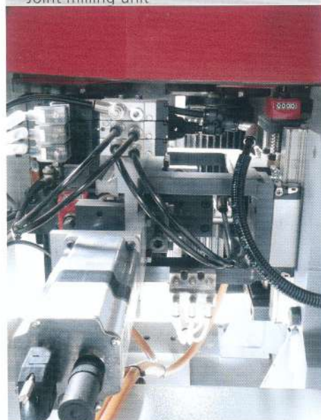
预铣修边单元 08.378 Joint milling unit
