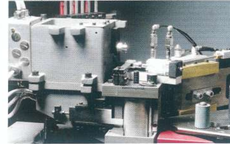
涂胶单元 04.1570 (Novimat R3) Edge banding unit (Novimat R3)
