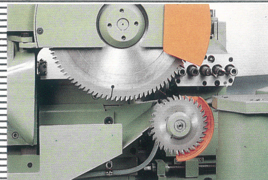
Incisore - Scoring unit - Inciseur Incisor - Vorritzer (optional)
